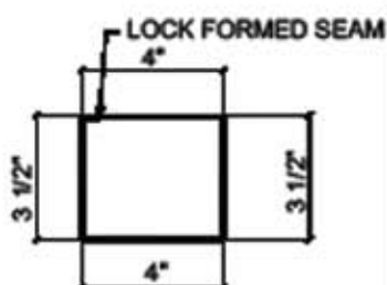
Downspout
